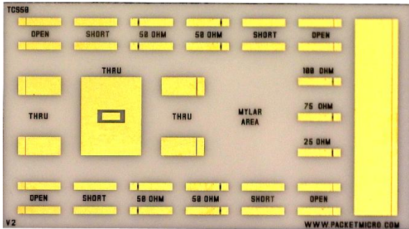
TCS50 Calibration Substrate
